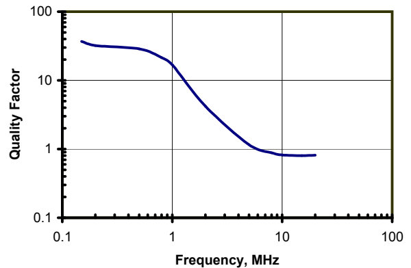
Quality Factor vs. Frequency
